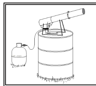
Figure 13. Propane exploder.
