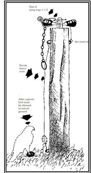
Figure 14. Padded-jaw pole trap.
